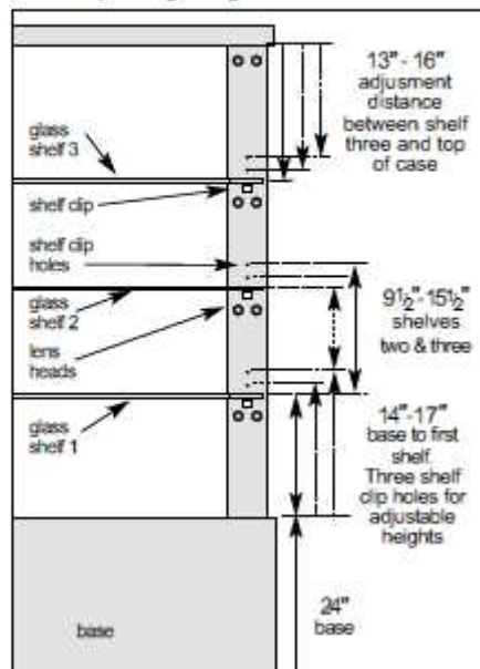
Showcase shown is a standard CM1 in Coppertex powder coated finish with solid metal back, powder coated with Charcoal finish.
